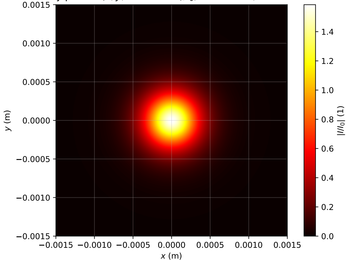
Intensity profile I(x, y, z = 2.866m)/I_0 , \text{Pin}=0.9\text{Pcr} , artificial time
